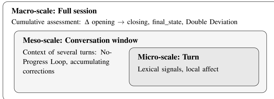
Figure 1: Three temporal scales of conversation analysis. The turn (micro) provides local signals; the conversation window (meso) reveals loops and building friction; the full session (macro) allows assessment of the cumulative relational outcome.
