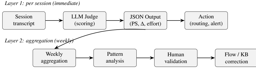
Figure 4: Two-layer action model. Layer 1 operates immediately per session (scoring → routing/alert). Layer 2 aggregates results weekly (e.g., topic clustering of turning-point triggers and reason codes (Grootendorst, 2022)) and requires human validation before implementing changes to the conversational flow or knowledge base.
