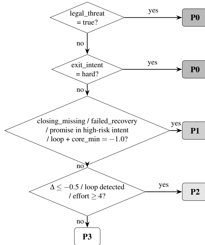
Figure 6: Priority Score (P0–P3) peak assignment decision tree, generated from the production rule engine. The closing band may additionally be reduced by at most one level under the closing_deescalation rule (Section 4.2). Sessions with a single customer turn bypass the tree and receive the “not measured” floor (insufficient_user_turns).
